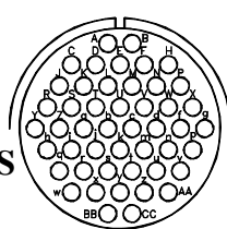
ARRANGEMENT 32-A48 CONTACT SIZE 16 SERVICE RATING I
